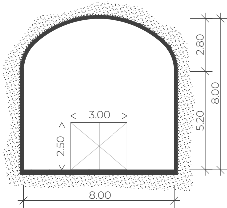
Cross-section
